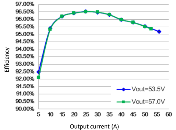
PIC 2 – EFFICIENCY (230VAC, 25°C)
