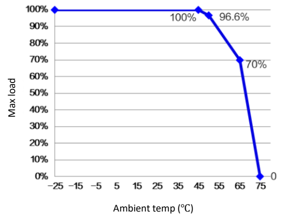
PIC 3 – POWER DERATING
